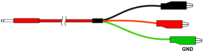
(1) PN # 400210A3RD Bantam to (3) Alligator Clips - Red, (6')
