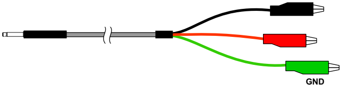
(1) PN # 400210A3BK Bantam to (3) Alligator Clips - Black, (6')
