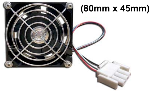
FTR UPN # TF-DCOMEF-01 48 Volt Replacement Fan for DCO MEF Bay w/ 3 Wire Plug
