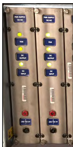
POWER SUPPLY (FRONT VIEW)
