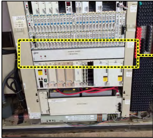
INSIDE VIEW OF 80A/D CABINET
