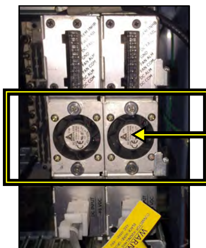
POWER SUPPLY (BACK VIEW) w/ EXISTING FANS
