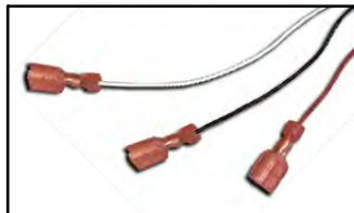
FTR UPN # TF-DCOCMF-01 48 Volt Fan for DCO CMF Bay w/ 3 Leads & Faston Connectors
