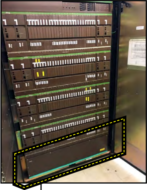
NT9X950 HAS (3) BLOWER UNITS PER BAY
