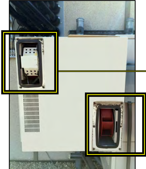
MESA XL CABINET DOOR w/ OLD FANS
