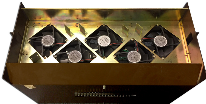
CONVERTED NORTEL DMS-100 NT3X90AA FAN UNIT * WITH (5) BRAND NEW 48VDC TAG FANS *(FAN UNIT IS NOT INCLUDED)
