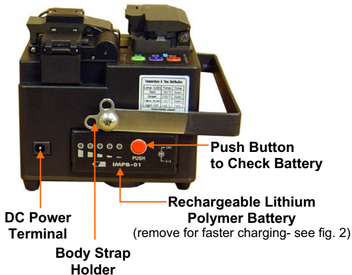
fig. 1 - Side View of Unit
