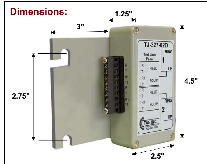
TJ-327-02D Test Jack Panel w/2 327C Jacks
