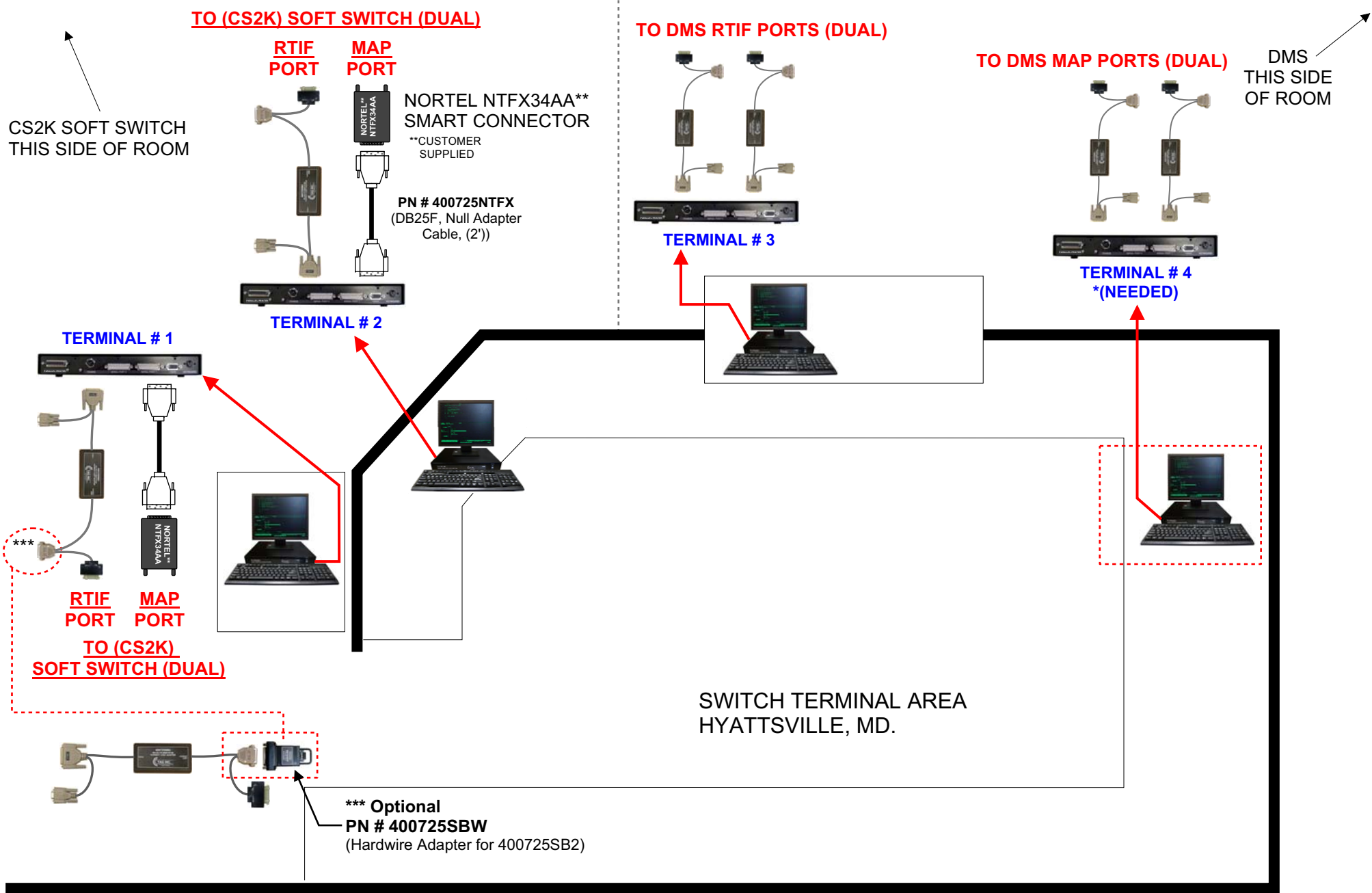
SWITCH CONTROL TERMINAL AREA SETUP AT HYATTSVILLE, MD. AS OF 2/15/2013
