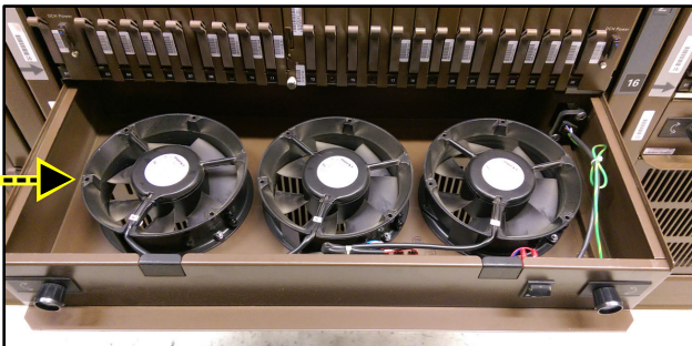
DMS-100 NTRX91AA FAN UNIT w/ EXISTING FANS
