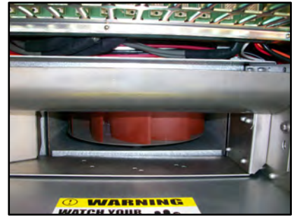
BOTTOM OF MESA CABINET w/ EXISTING FAN (ORDER PN # TF-MC225-02)
