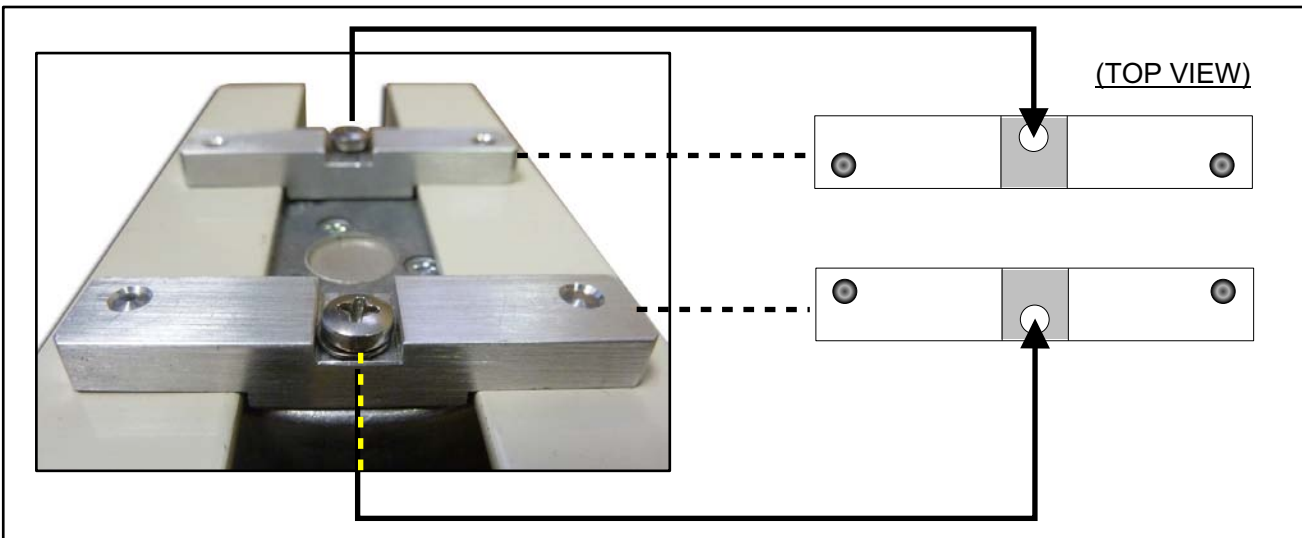
FIGURE 5, TOP VIEW DETAIL
