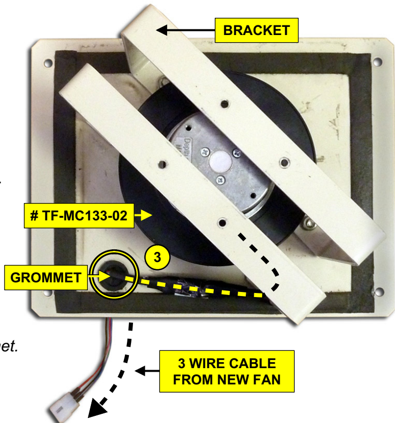
FIGURE 2, TF-MC133-02 WIRE DRESSING DETAIL
