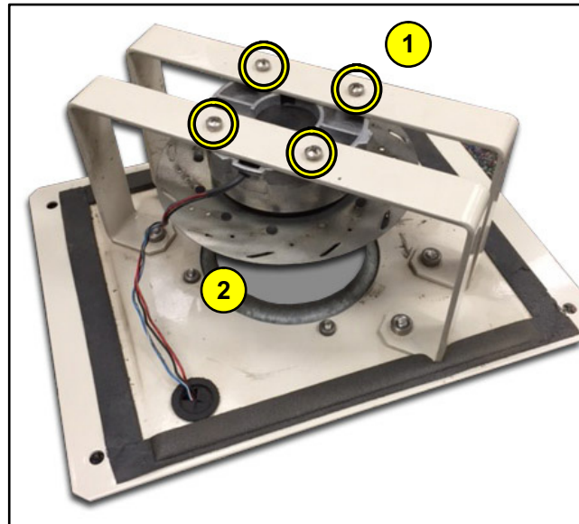
FIGURE 1, EXISTING BRACKET w/ OLD FAN
