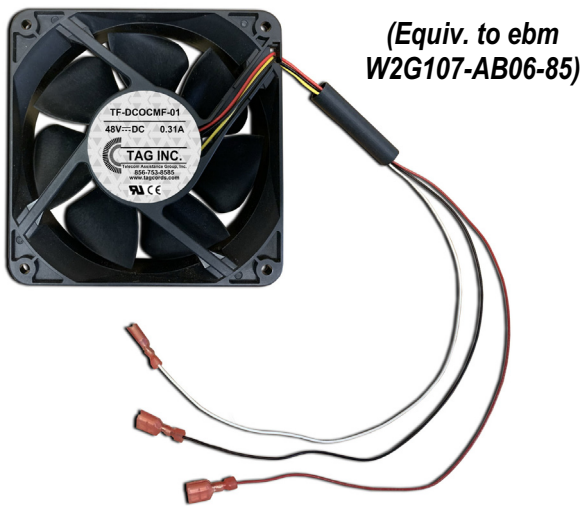
PN # TF-DCOCMF-01 48 Volt Replacement Fan for DCO CMF Bay w/ 3 Leads & Faston Connectors
