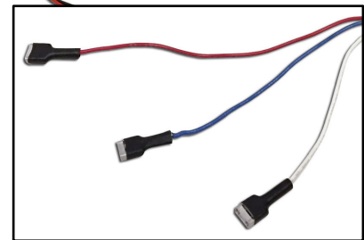
PN # TF-DCO-02 48 Volt Replacement Fan for DCO CMF / DTF Bay w/ 3 Leads & Faston Connectors (fan only - use with existing guard grill)
