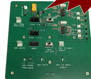
BUILT IN SENSOR CONTROL (NO PADDLES) Fan Control Board w/ built in Sensors (no paddles needed)
