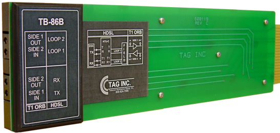
WINBUY # TB86B "DDM Plus" Office Repeater Test Board w/ Bantam Jacks
