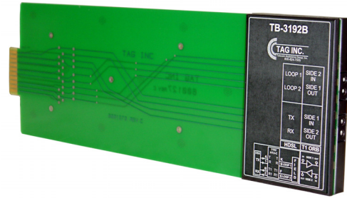
WINBUY # TB3192B 3190/3192 Office Repeater Test Board w/ Bantam Jacks
