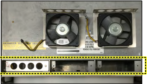
VORTEX RECTIFIER FAN UNIT w/ EXISTING FANS (V200E50 type w/ (3) separate trays)
