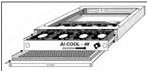
AICOOL-48 FAN UNIT (8 FANS) (fan tray unit is not included)
