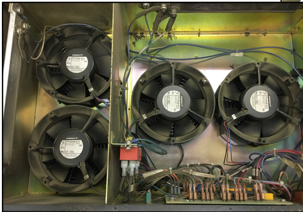
TOP VIEW OF DCO RLS CABINET FAN TRAY (tray has (4) fans)
