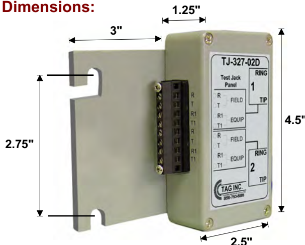
TJ-327-02D Test Jack Panel w/ (2) 327C Jacks
