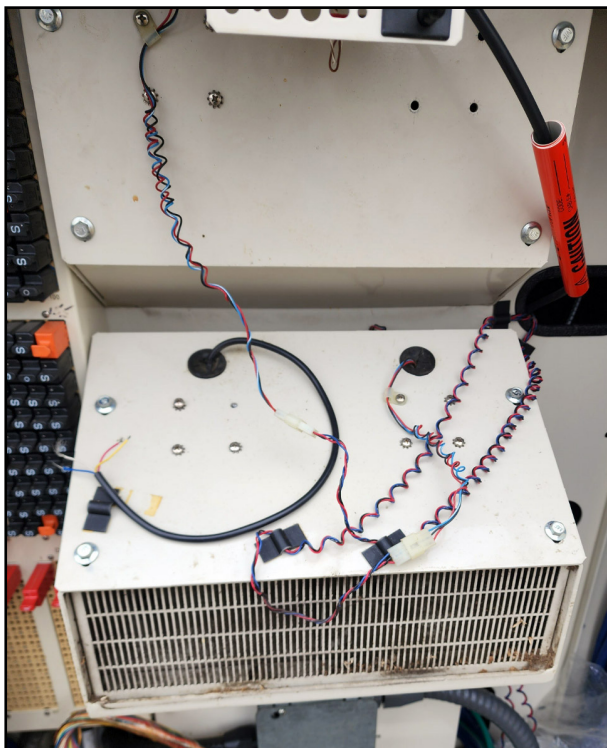
INSIDE VIEW OF MESA 768 CABINET (DUAL FAN HOUSING)
