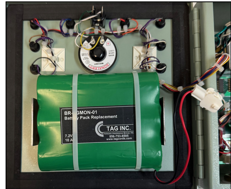
INSIDE VIEW of NEW NIMH BATTERY PACK 7.2V, 10Ah 72Wh, 3X
